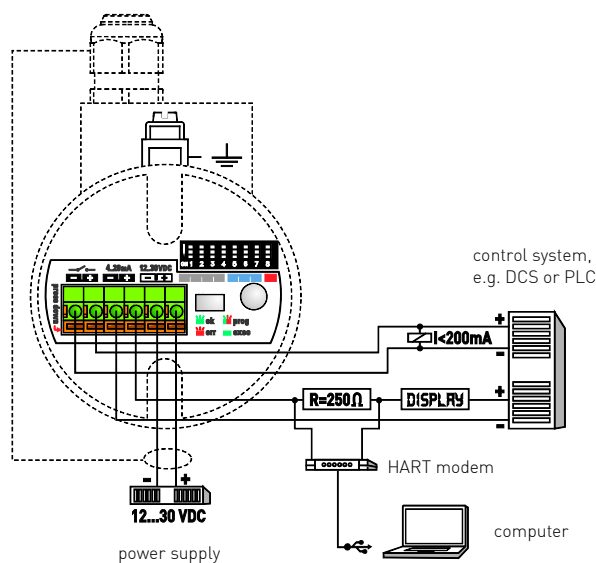
Figure 9: electrical connection
