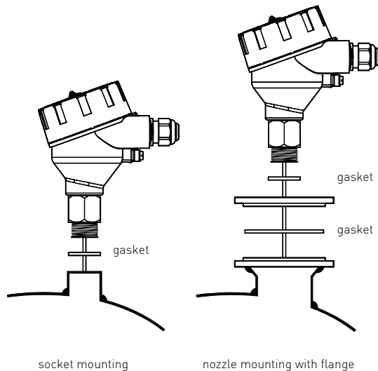
Figure 7: mounting
