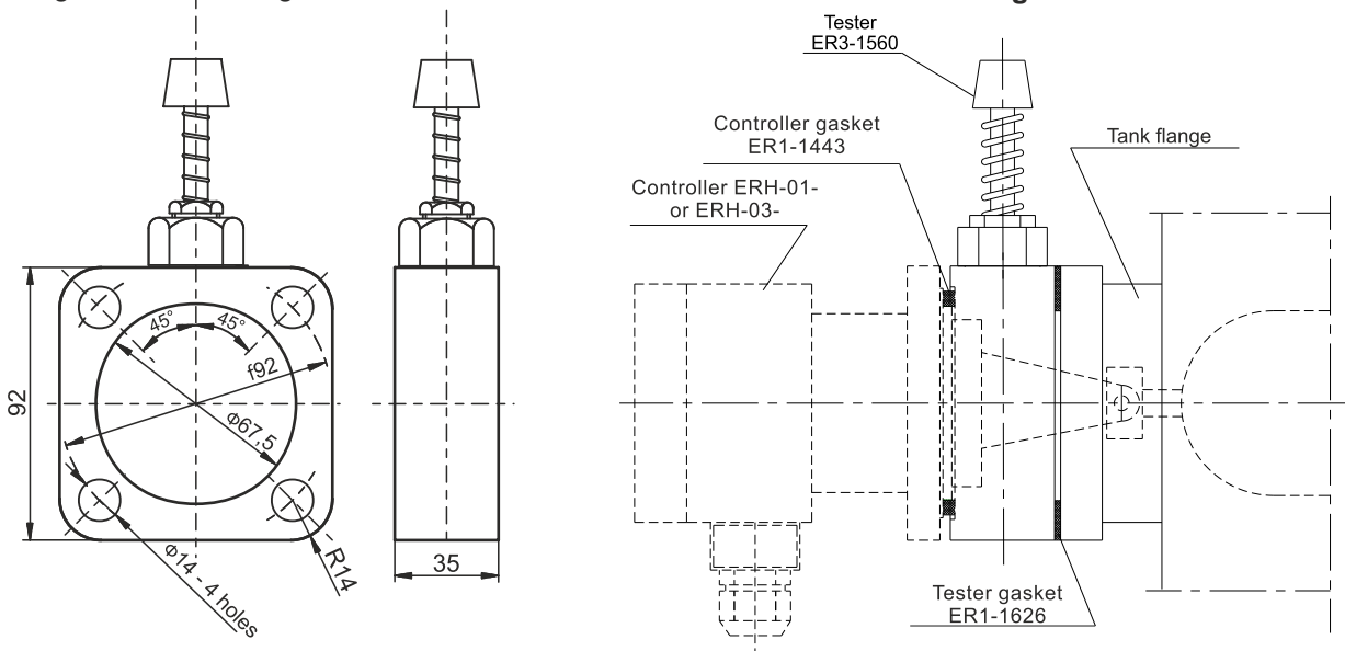
Example of the controller mounting with the tester ER3-1560
