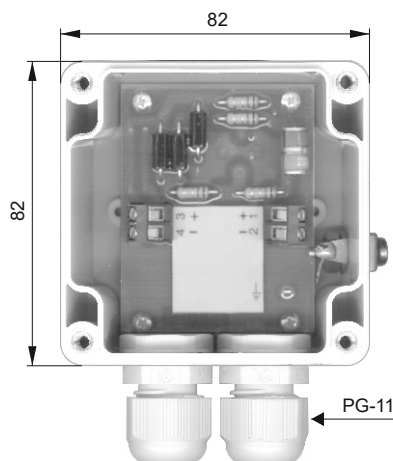
Wall-mounted version
