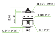
YT-400S, YT-405S(Single Acting)
