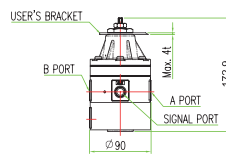
YT-430S, YT-435S (Single Acting)
