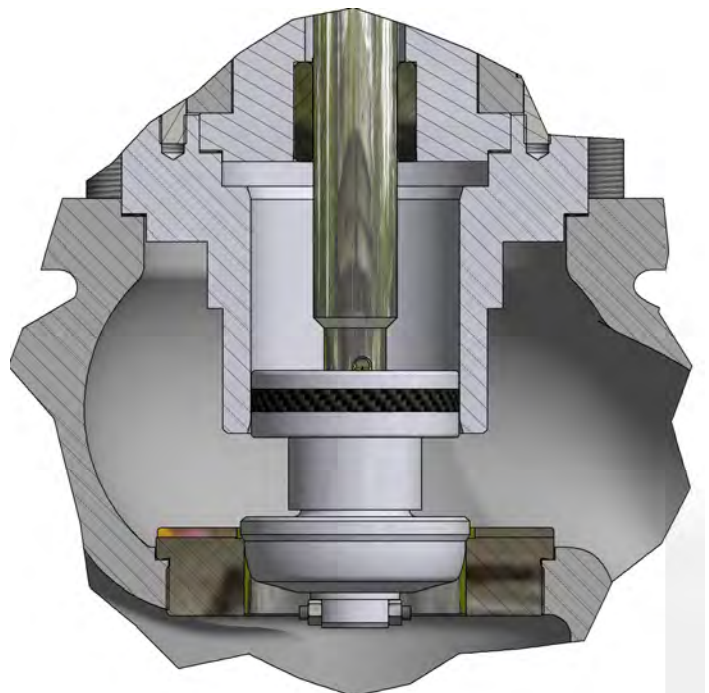
BALANCED TRIM
